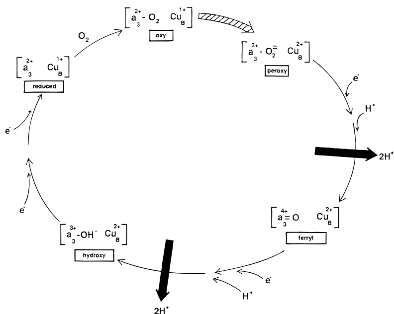
Figure 6. Simplified reaction scheme for oxidation of reduced cytochrome oxidase by dioxygen. The reduced binuclear center reacts with O_2 to form an oxy intermediate, which undergoes successive one-electron reductions to form peroxy and ferryl intermediates, respectively. These latter two electron transfers are coupled to proton translocation, as indicated by the heavy, shaded arrows. The structures of the intermediates are used only for an electron count and are not intended, necessarily, to represent actual, proposed structures.
