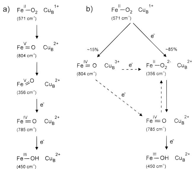
Figure 10. Alternative structural proposals for the oxygen isotope sensitive vibrations that are observed during the reaction of cytochrome oxidase with dioxygen in time-resolved resonance Raman measurements. Reaction sequences and the observed vibrational frequency and postulated structure for each of the intermediates are shown. Part a summarizes a recent model presented by Kitagawa and co-workers (see ref 96 and the text for details). Part b presents suggested structures in a reaction sequence proposed by Babcock and co-workers (see ref 48 and the text for details).
