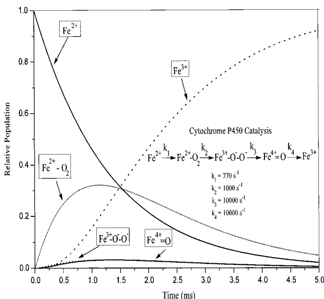
Figure 4. Concentration versus time profiles for various intermediates in the P450 reaction cycle with mechanism and rates as indicated.
